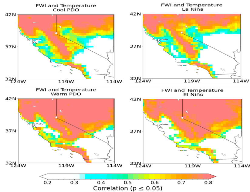
Figure 12. Correlation between FWI and 2 m temperature ( ^{\circ}\text{C} ) during cool (top) and warm (bottom) PDO (left) and La-Niña (top) and El Niño (bottom) ENSO (right) phases. Dark orange shading represents strong positive correlation.
