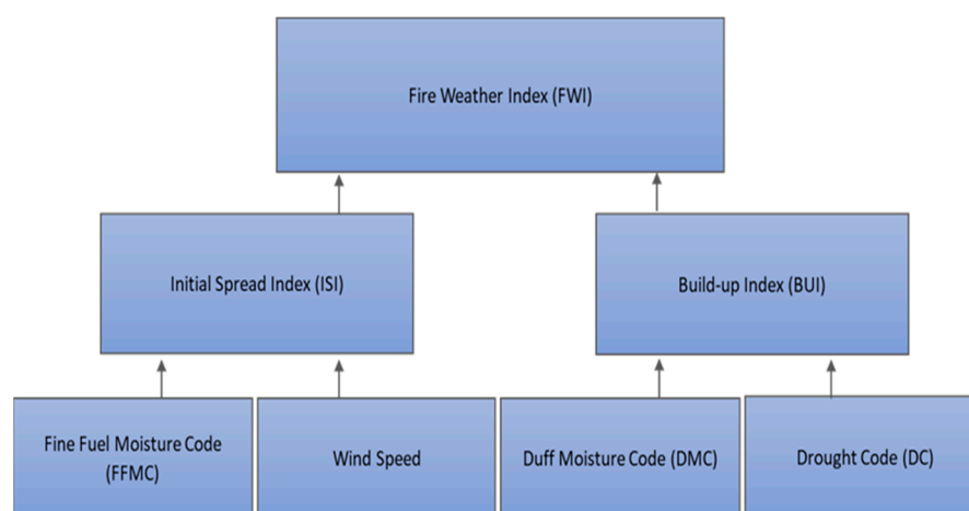
Figure 1. Flowchart illustrating how the FWI is calculated from the initial spread index and the build-up index. The ISI combines the FFMC and wind speed to calculate the estimated rate of fire spread. The ISI value usually doubles when the wind speed increases by 13 km/h [54]. The BUI, on the other hand, is a weighted combination of the DMC and DC that indicates the total amount of fuel accessible for burning by moving a flame front.
