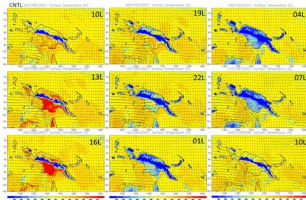
Figure 8. The 3-hour surface temperature and 900 mb winds for the CNTL case. (L denotes the local time on the island)
