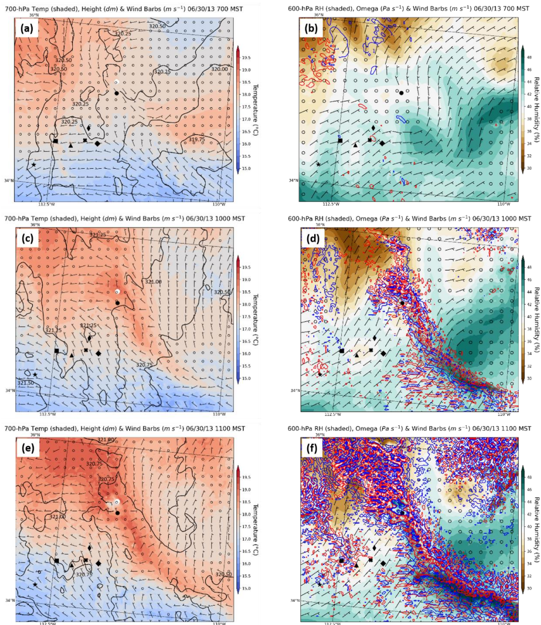
Figure 16. WRF-ARW-simulated 2.3-km meso- \beta -scale 700-hPa temperatures (red dashed in °C), isoheights (solid in dam), and wind barbs ( m s^{-1} ) and 600-hPa omega (red- and blue+ = solid in \mu b s^{-1} ), wind barbs ( m s^{-1} ), and 600-hPa relative humidity (fill in %) valid at (a,b) 1400 UTC, (c,d) 1700 UTC, and (e,f) 1800 UTC 30 June 2013. Icons are place locators as in Figure 3a.
