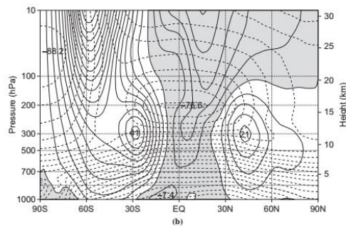
FIGURE 6.1 Meridional cross-sections of longitudinally and time-averaged zonal wind (solid contours, interval of 5 \text{ m s}^{-1} ) and temperature (dashed contours, interval of 5 K) for December-February (a) and June-August (b). Easterly winds are shaded and 0^\circ\text{C} isotherm is darkened. Wind maxima shown in \text{m s}^{-1} , temperature minima shown in ^\circ\text{C} . (Based on NCEP/NCAR reanalyses; after Wallace, 2003.)
