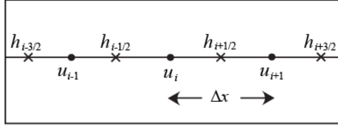
Fig. 13.5: A schematic of a staggered grid mesh for the shallow water system.
