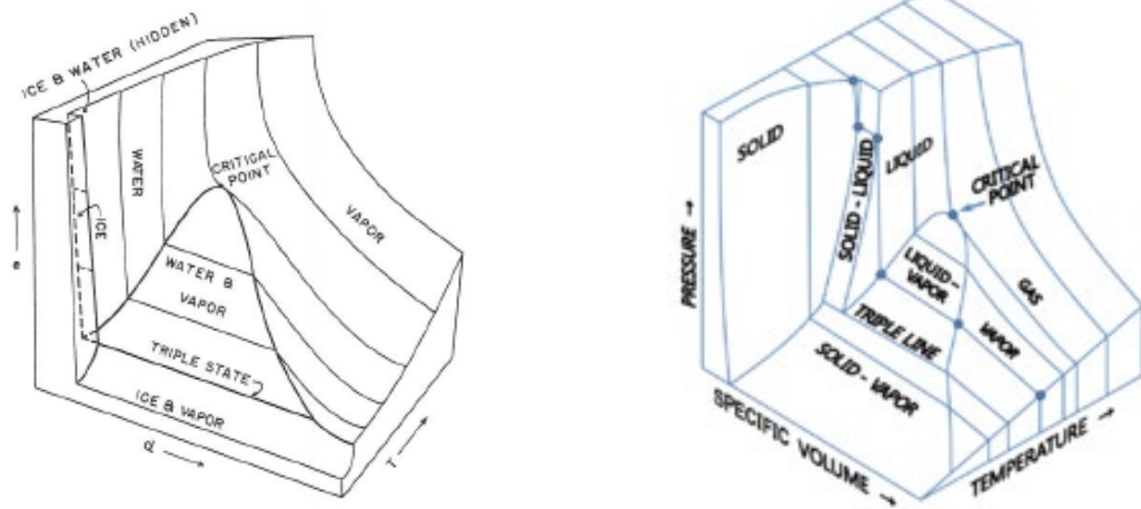
Figure 4.4: (Hess) 3D thermodynamic surface of water substance.
